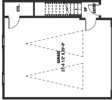
MAIN FLOOR PLAN RESIDENTIAL SPACE: 624 SQ.FT
