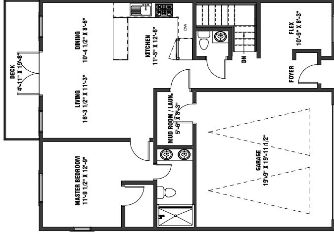
MAIN FLOOR PLAN RESIDENTIAL SPACE: 887 SQ.FT
